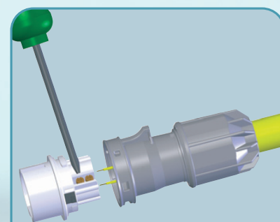
open contact screws
